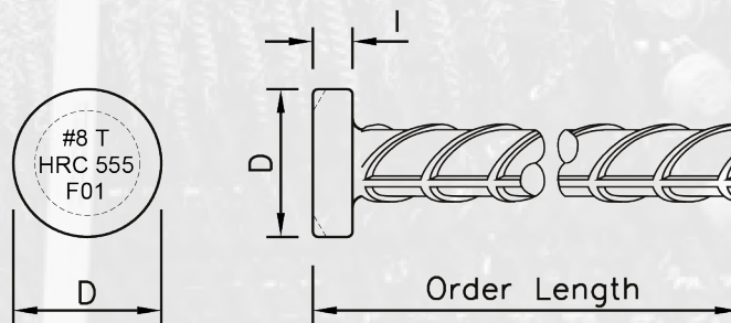
Dimensions of HRC 555 Series T-Head
